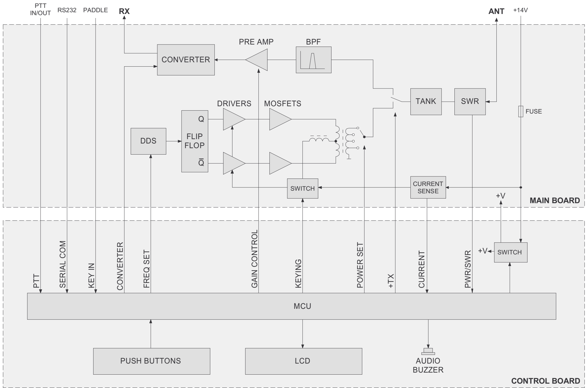
JUMA TX500 block diagram 2009-08-02 OH2NLT & OH7SV
